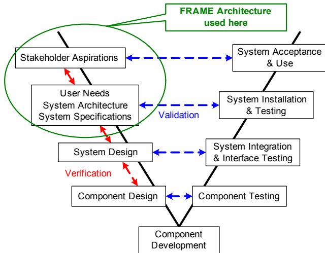
Figure 1 – V-model system lifecycle
